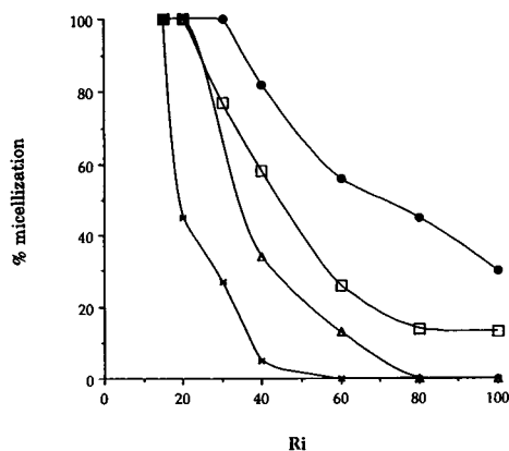
FIGURE 3 Percentage of micellization as a function of the lipid/peptide ratio ( R_i ) obtained at 26°C, pH = 7.5 for (□) pure DPPC, (●) DPPC/10(mol)% palmitic acid, (△) DPPC/10(mol)% oleic acid, and (*) DPPC/10(mol)% linoleic acid.
