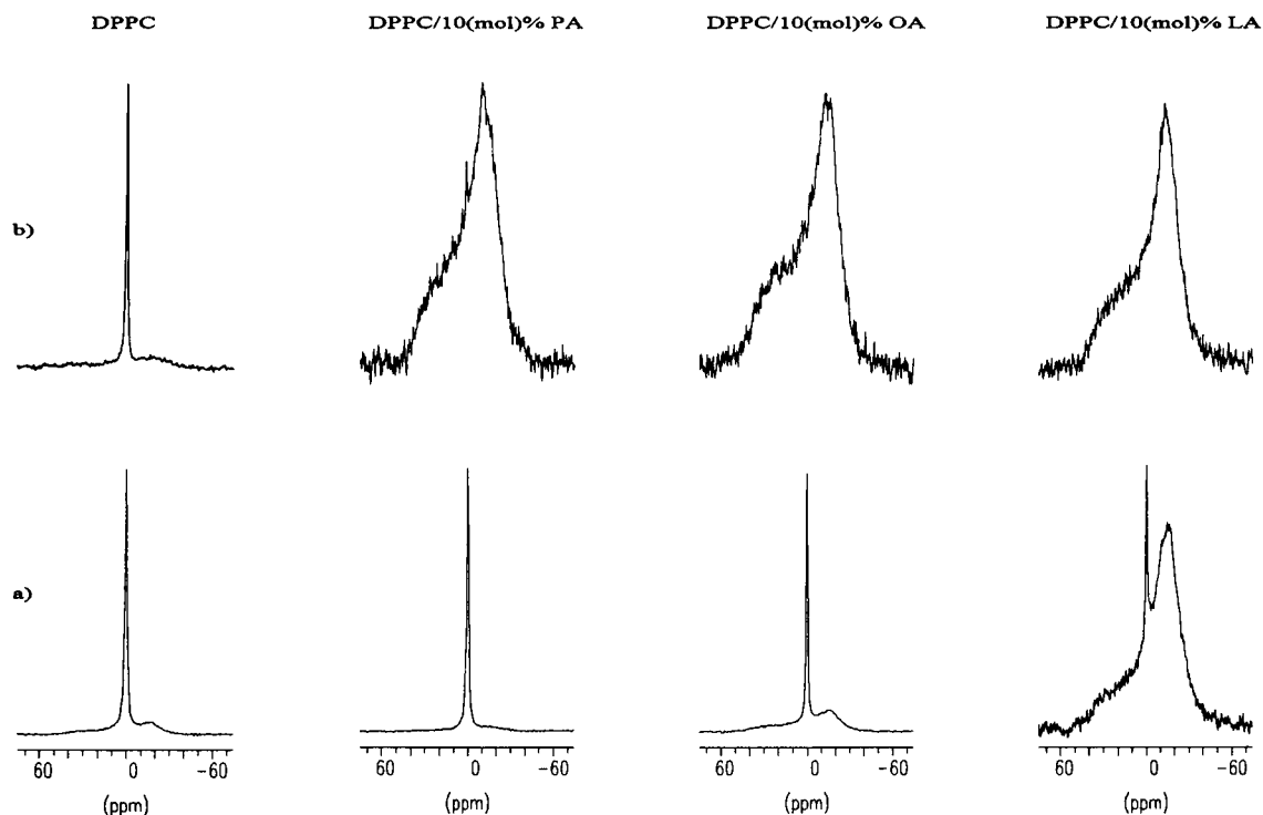
FIGURE 1 ^{31}\text{P} NMR spectra of samples containing 10(mol)% of palmitic, oleic, or linoleic acid compared to pure DPPC, in the presence of melittin ( R_i = 40 ), at 26^\circ\text{C} . (a) pH = 7.5; (b) pH = 9.5. The sample composition is indicated at the top of each column.
