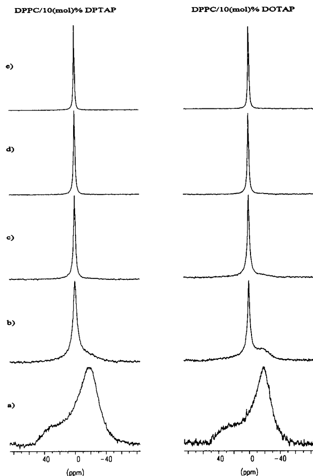
FIGURE 4 ^{31}\text{P} NMR spectra of DPPC samples containing 10(mol)% of DPTAP or DOTAP, at 26°C, pH = 7.5 (a) without melittin and (b–e) in the presence of melittin: (b) R_i = 100 ; (c) R_i = 60 ; (d) R_i = 40 ; (e) R_i = 30 . The sample composition is indicated at the top of each column.
