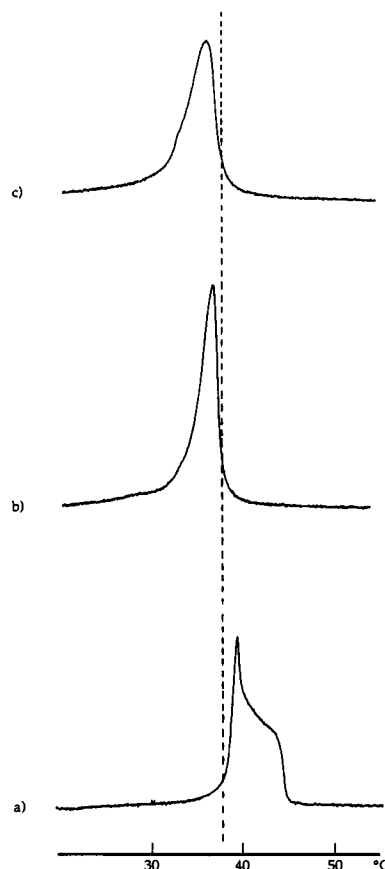
FIGURE 5 Differential scanning calorimetry traces for DPPC- \text{d}_{62} samples containing 10(mol)% of (a) palmitic acid, (b) oleic acid, and (c) linoleic acid. The scan rate was 10°C/h. The dotted line represents the transition temperature for pure DPPC- \text{d}_{62} : 37.7°C (Vist and Davis, 1990).
